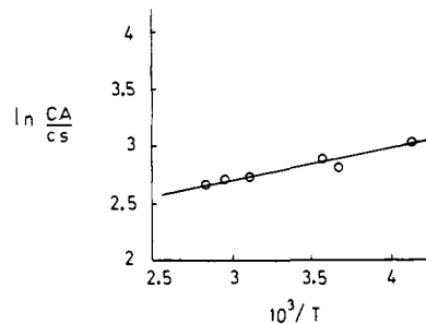
Figure 2. Arrhenius plot for the pair of products 4 (CA) and 5 (CS) formed from deazetation of 2a,b ( r = 0.965 ).
